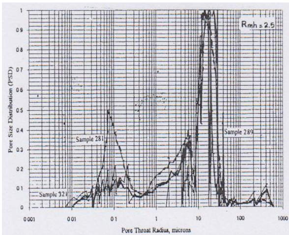
Figure 9. Pore throat size distribution plot for HU 3.
