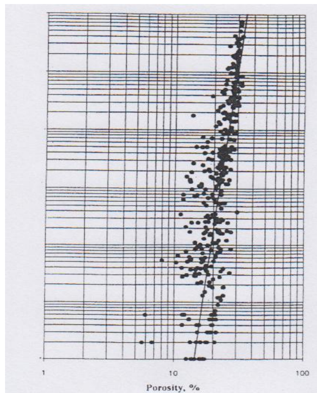
Figure 5. Log porosity versus log permeability.
