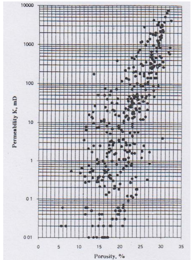
Figure 4. Porosity versus log permeability.
