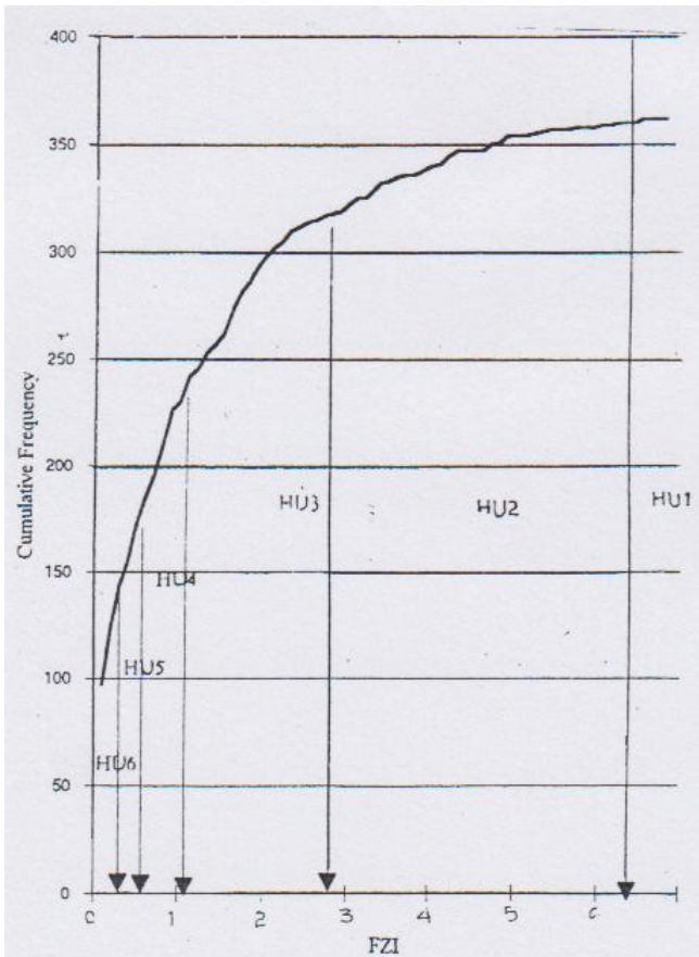
Figure 3. FZI versus cumulative frequency (interval = 0.15).
