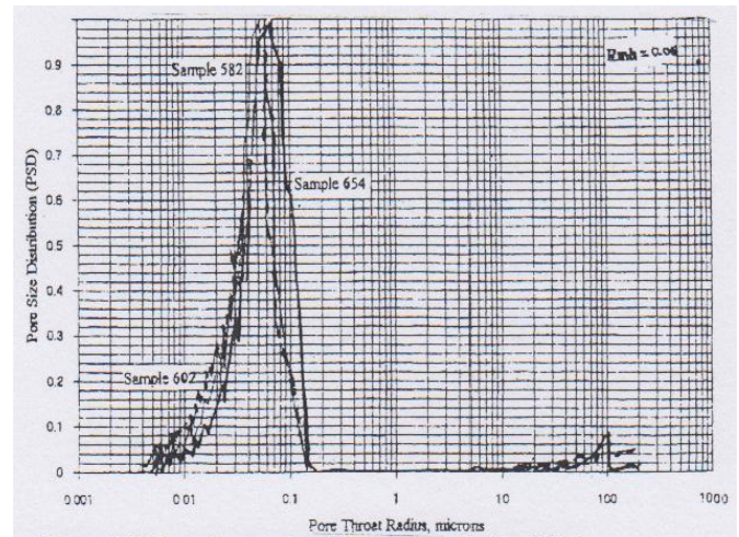
Figure 12. Pore throat size distribution plot for HU 6.
