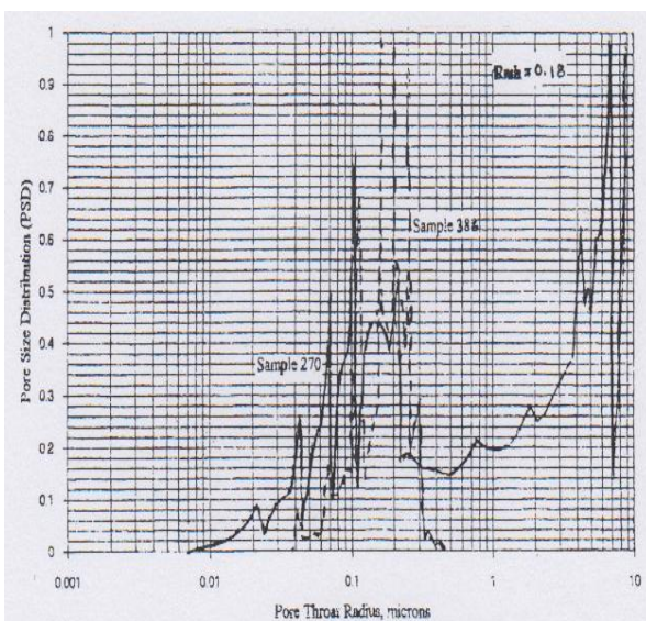
Figure 11. Pore throat size distribution plot for HU 5.
